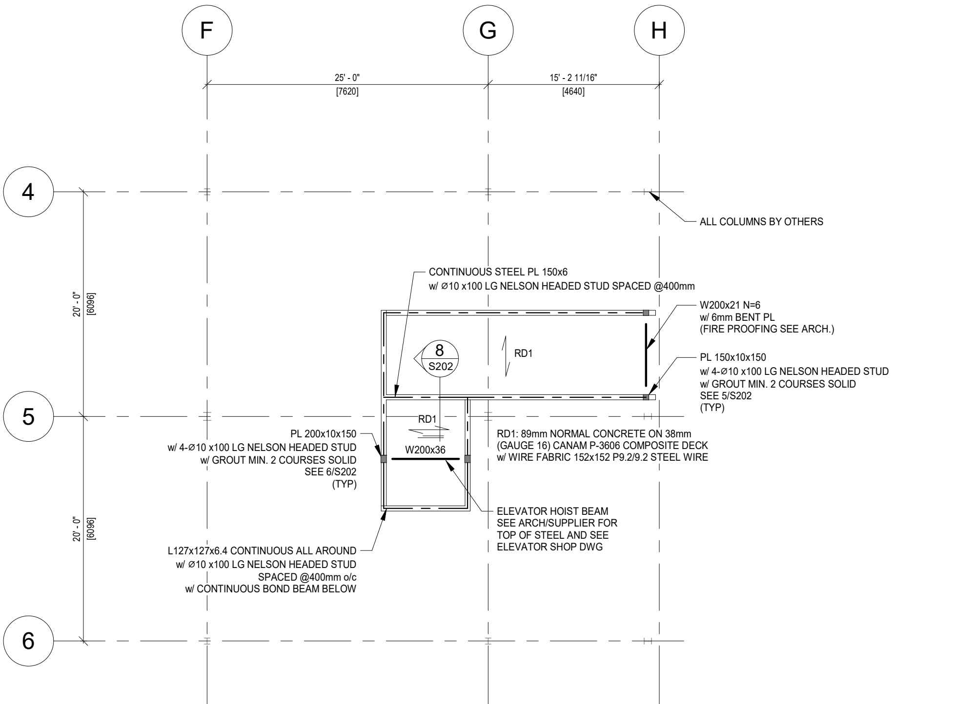
4 ROOF OF STAIRWELL A AND ELEVATOR S202 1 : 100 NOTE: SEE ARCH. DRAWING FOR TOP ELEVATION
